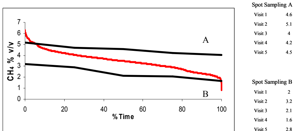
Figure 5. Concentration duration curves for CH 4 . The red line is constructed from the high frequency continuous data and the black lines compiled from random samples taken from the continuous data set to represent conventional periodic weekly sampling (see spot sampling A and B).
