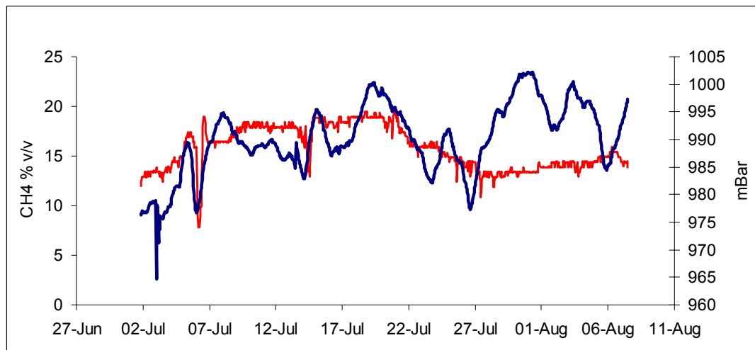
Figure 7. In this continuous data set the expected relationship between atmospheric pressure and concentration does not exist. Between 2 – 22 nd July the inverse relationship is observed i.e, when pressure increases the concentration increases.
