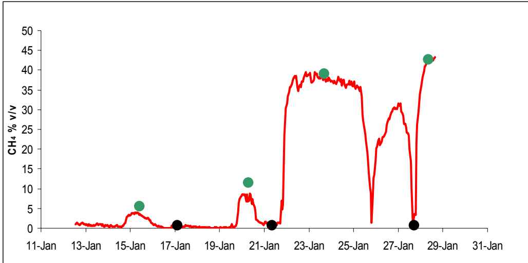
Figure 2. Continuous gas concentration data from “The Christmas Borehole”, a landfill perimeter borehole thought to indicate gas migration problems only at Christmas time. A period of continuous data collection has overcome the artefact arising from the sampling frequency (monthly) mismatching with the variability of concentration. The continuous data clearly showed that though the CH 4 concentration is variable it is not only high at Christmas. Collecting spot samples on days with the green dots compared to days with the black dots would result in an extremely different perception of risk.
